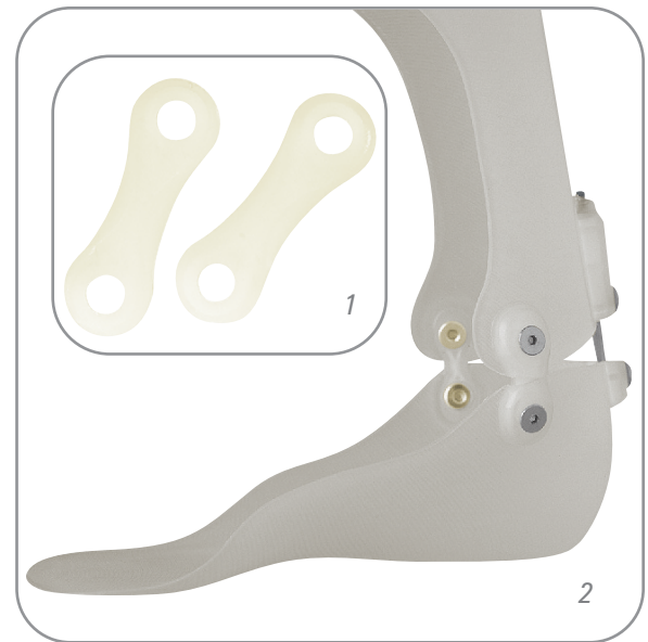
1 = Model 740 - Tamarack Flexure Joint® 2 = Model 740 used on a molded AFO
