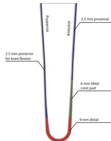
Alpha Silicone Liner (Select Fabric) Progressive Style
